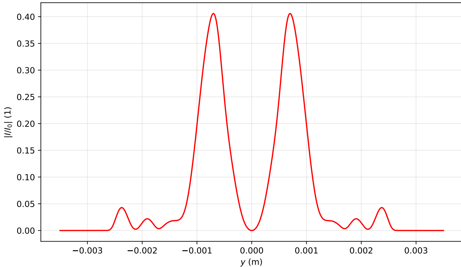
Intensity profile I(x=0, y, z=3.025)/I_0 , \text{Pin}=6.0\text{Pcr} , artificial time
